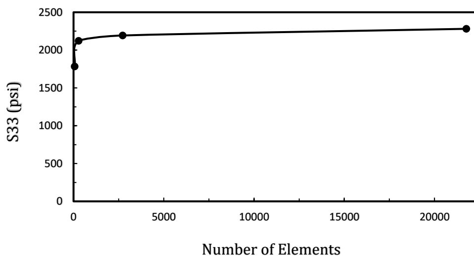
Mesh Sensitivity Analysis
